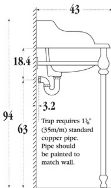
Three-hole 22" Basin.
