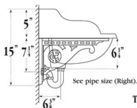
22" Lavatory Basin.
