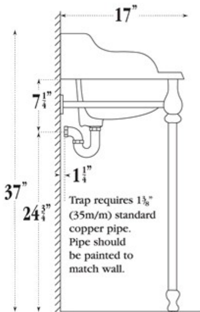
22" Lavatory Basin.
